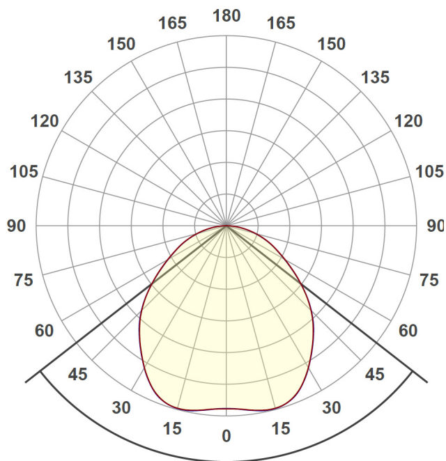
Beam angle: 104,1° Intensity distribution - Polar
